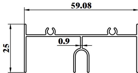
SW696A WEIGHT : 0.384 KG/M AP : 307.38mm
