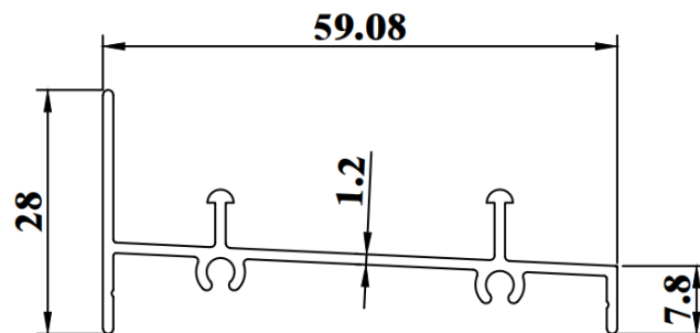
SW936G WEIGHT : 0.412 KG/M AP : 245.38mm
