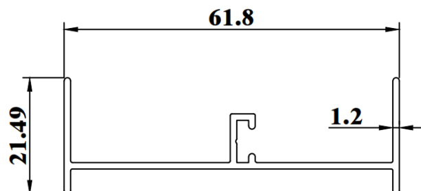
SW697G WEIGHT : 0.382 KG/M AP : 234.82mm
