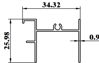
SW078A WEIGHT : 0.245 KG/M AP : 194.25mm
