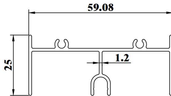
SW696G WEIGHT : 0.496 KG/M AP : 297.37mm
