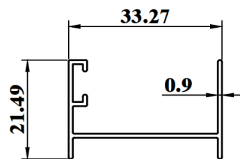
SW077A WEIGHT : 0.203 KG/M AP : 166.54mm
