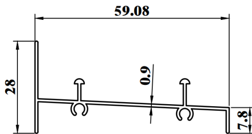
SW 936A WEIGHT : 0.313 KG/M AP : 250.82 mm
