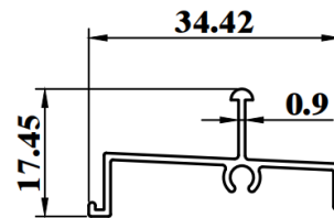
SW076A WEIGHT : 0.175 KG/M AP : 132.16mm
